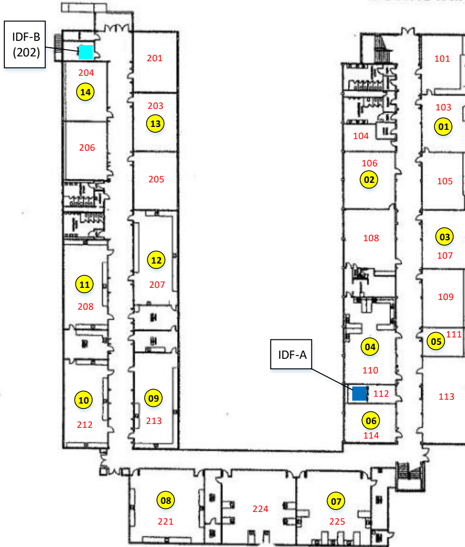
100 BLDG. DOWNSTAIRS
