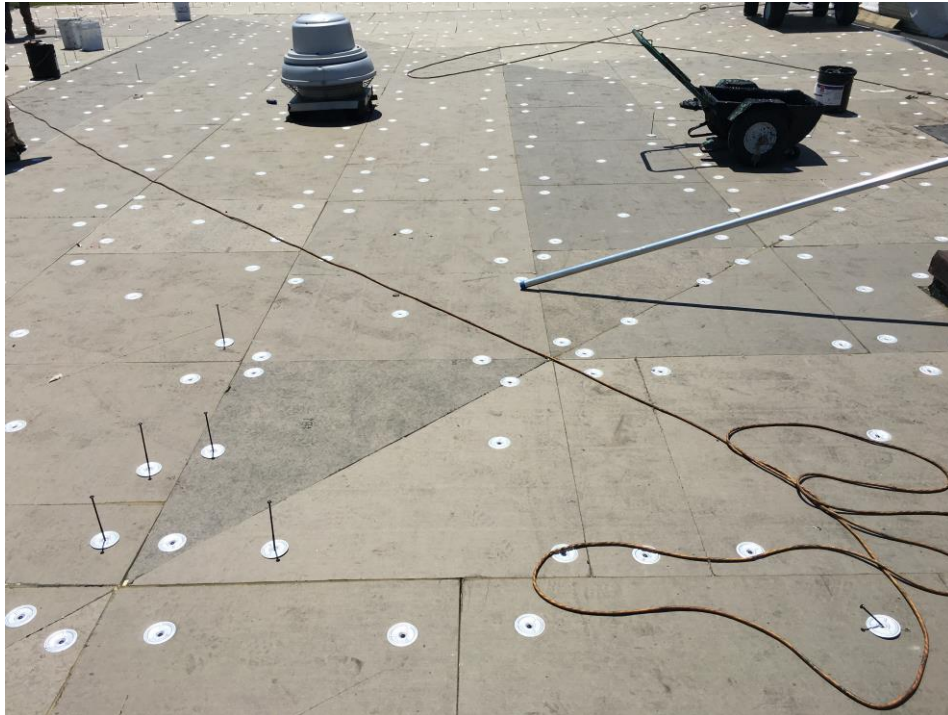
June 2018: Belleville HS – new tapered insulation being installed over metal deck.
