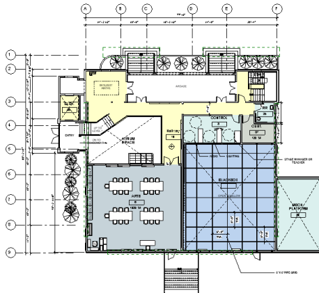
Level 1
