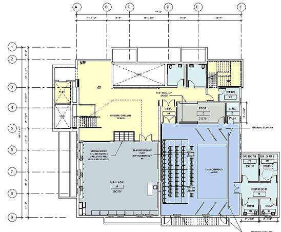
Level 2
